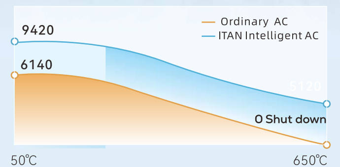
Cooling Capacity Comparison (Btu/h)
