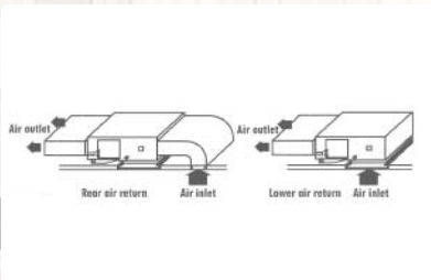
Medium Static Pressure (100Pa) 36k/42k/48k/60k BTU/h
